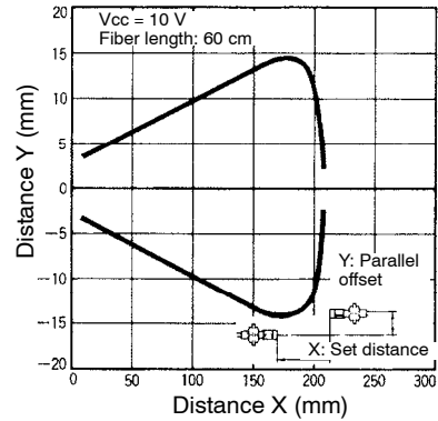
EE-SPZ301/SPZ401 with E32-TC200 and E39-F1
