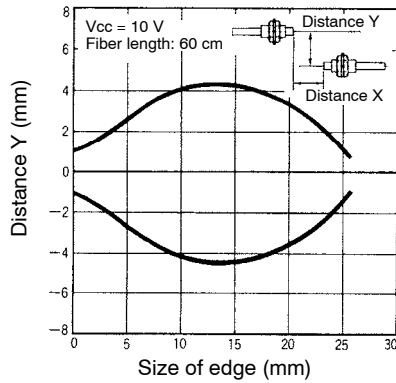
EE-SPZ301/SPZ401 with E32-TC200 and E39-F2
