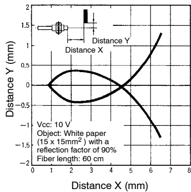
EE-SPZ301/SPZ401 with E32-DC200
