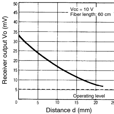
EE-SPZ301/SPZ401 with E32-TC200 and E39-F2
