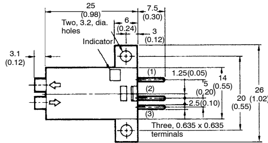
Terminal Arrangement
