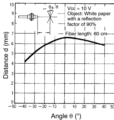
EE-SPZ301/SPZ401 with E32-DC200
