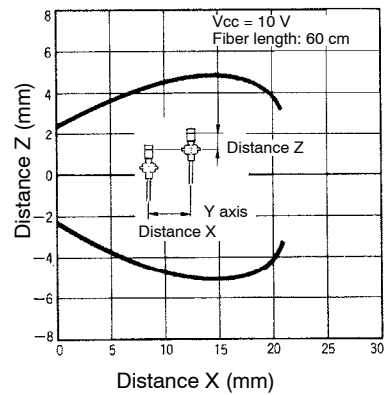
EE-SPZ301/SPZ401 with E32-TC200 and E39-F1
